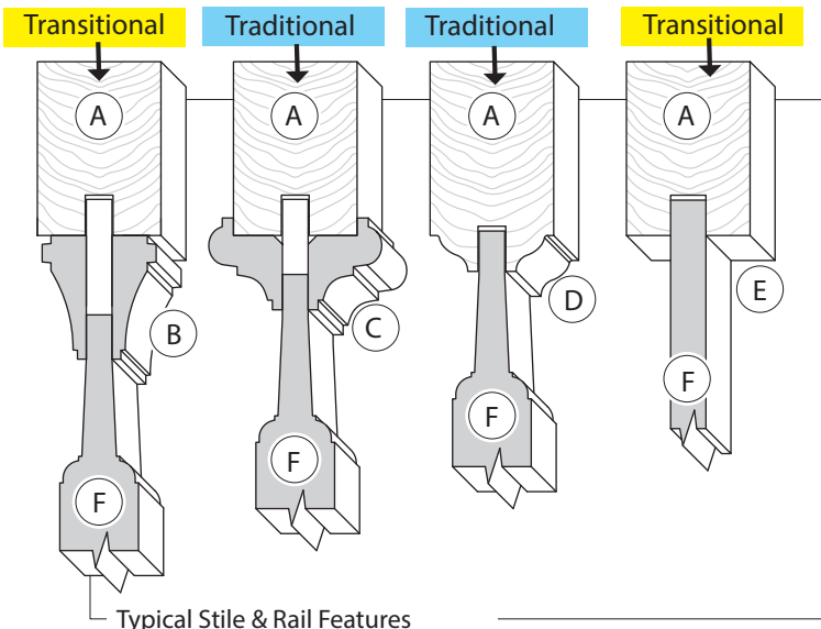
Typical Stile & Rail Features
